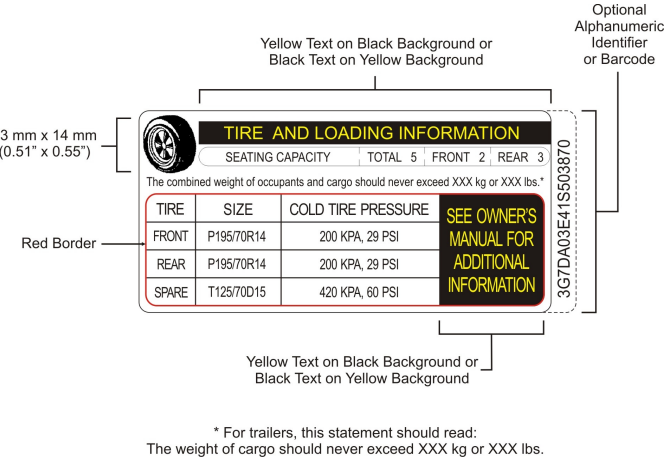
Figure 1 — Vehicle Placard, Unilingual English Example
