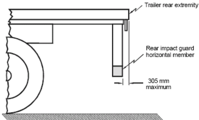
Figure 1 — Side View of Trailer
