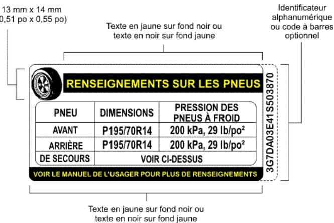
Figure 5 — Tire Inflation Pressure Label, Unilingual French Example
