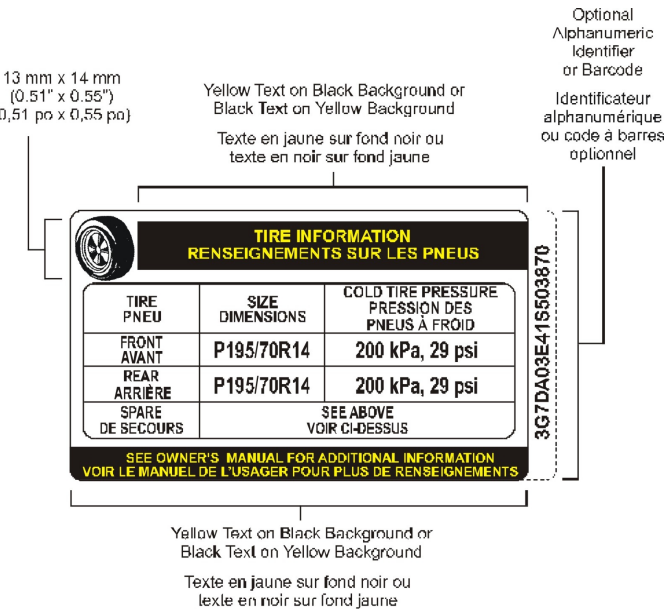
Figure 6 — Tire Inflation Pressure Label, Bilingual Example
