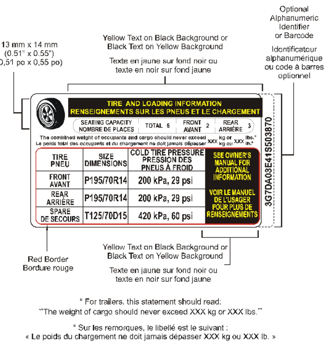
Figure 3 — Vehicle Placard, Bilingual Example
